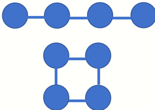
Figure 2: A path and a cycle.
